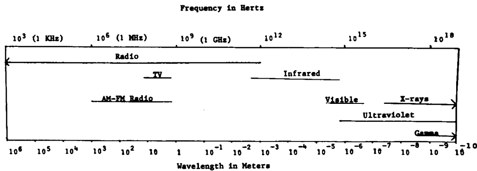
FIGURE G-1.—The electromagnetic spectrum.
